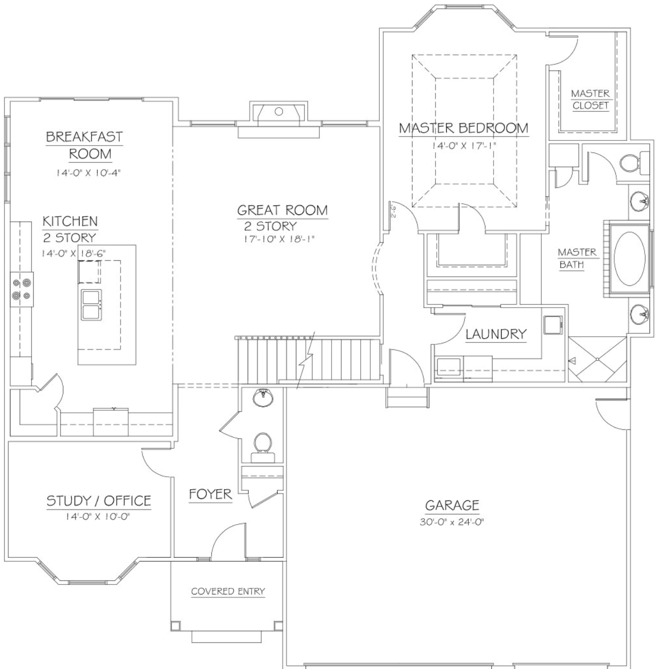
FIRST FLOOR PLAN 1871 S.F
