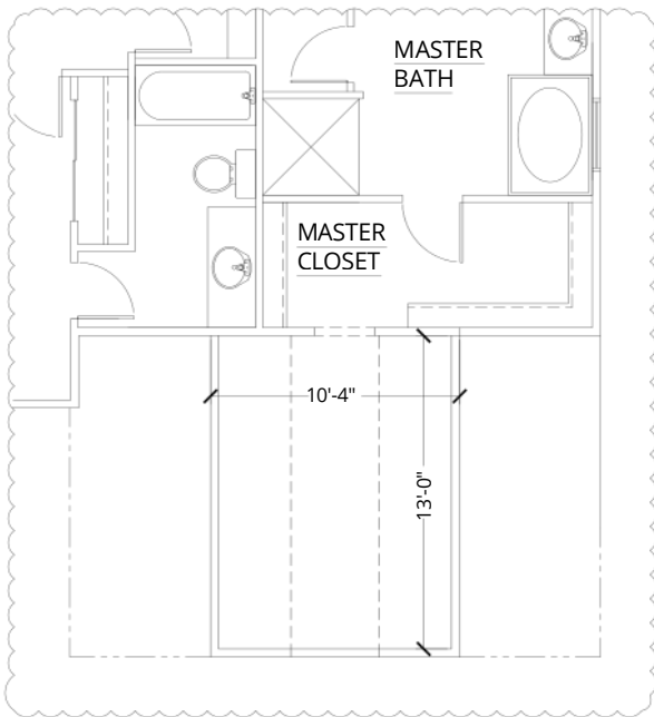
EXPANDED MASTER CLOSET OPTION FRONT LOAD GARAGE ADDS 130 S.F.
