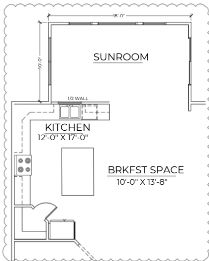
SUNROOM OPTION 180 S.F.
