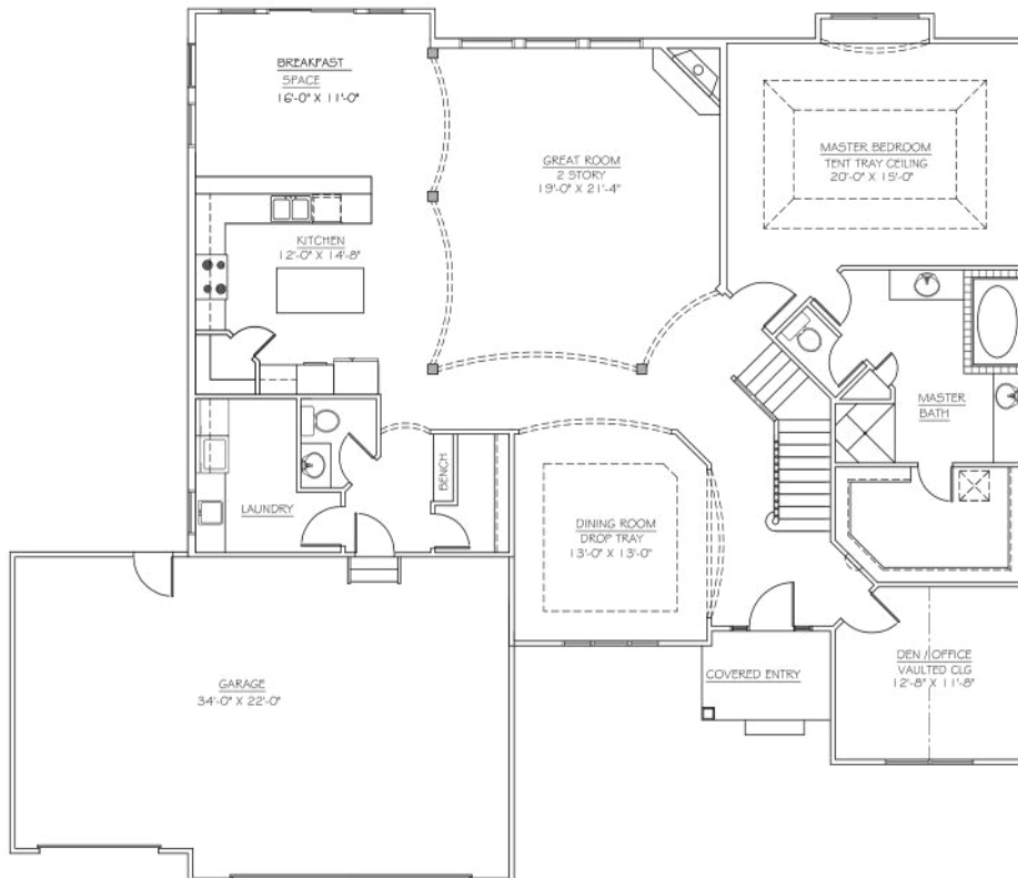
FIRST FLOOR PLAN - ELEVATION #2
