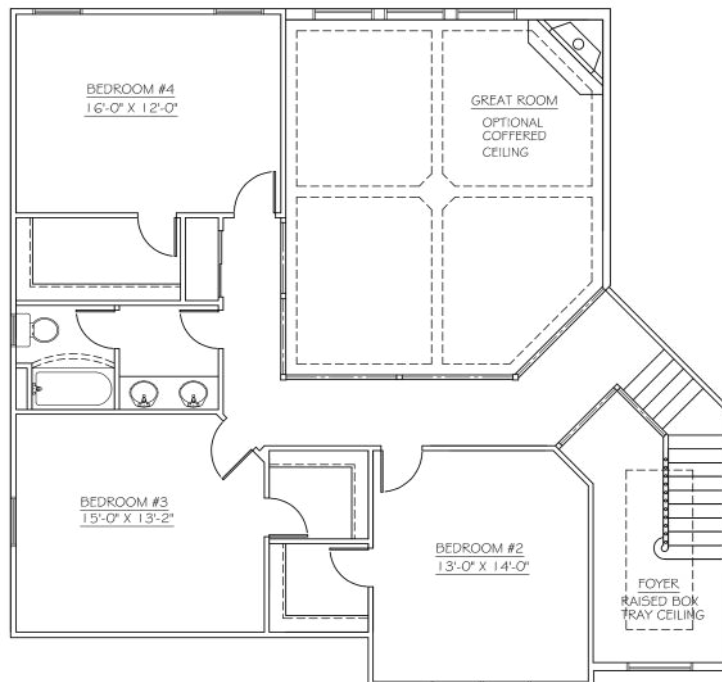
SECOND FLOORPLAN OPTION ALL ELEVATIONS
