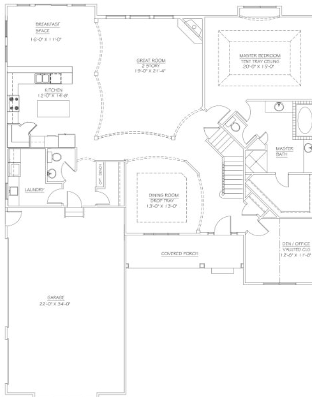
STANDARD FIRST FLOOR PLAN - SIDE LOAD GARAGE
