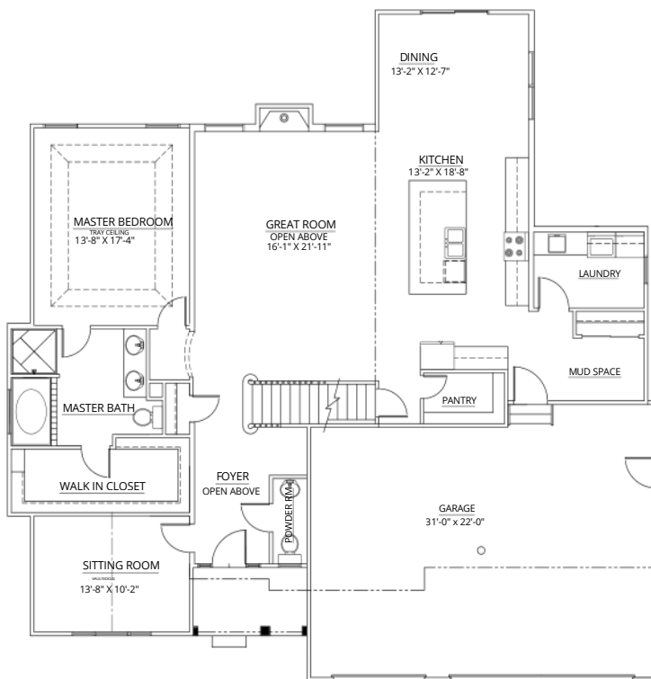
FIRST FLOORPLAN OPTION 1ST FLOOR = 1864 S.F.
