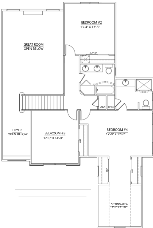
SECOND FLOOR PLAN OPTION #2 SIDE LOAD GARAGE ONLY 1144 S.F.
