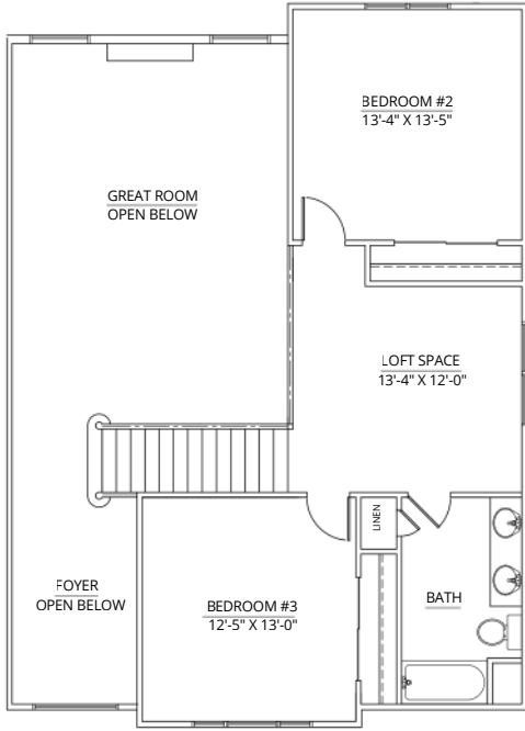
SECOND FLOOR PLAN OPTION #4 709 S.F.
