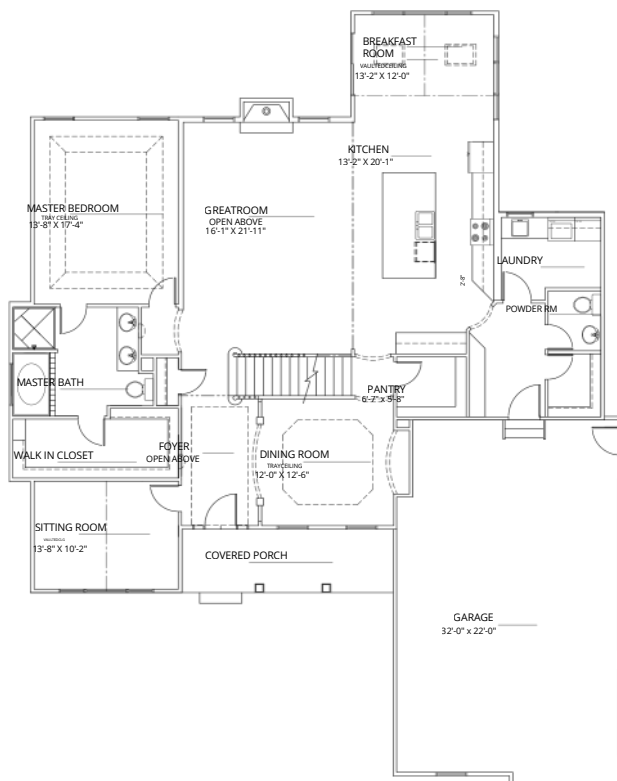
FIRST FLOORPLAN OPTION - SIDELOAD GARAGE 1ST FLOOR = 2096 S.F.
