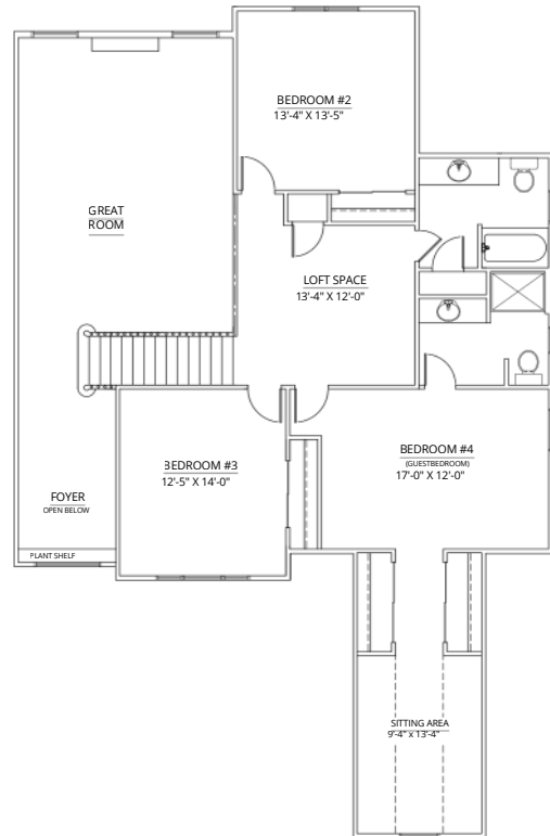
SECOND FLOOR PLAN OPTION #3 SIDE LOAD GARAGE ONLY 1221 S.F.
