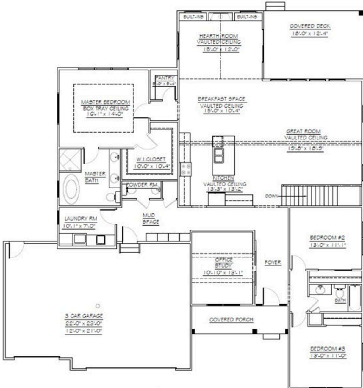
MAIN FLOOR PLAN 2448 S.F.
